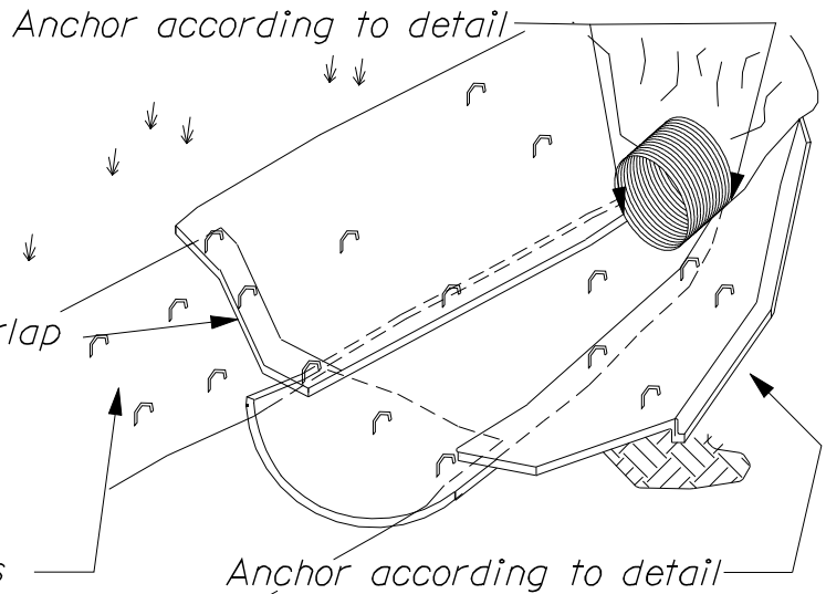
~ COVERED CHANNEL SIDE SLOPES ~
