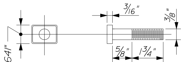
Post clip bolts shall be stainless steel on all overhead signs
