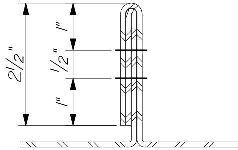
J Seam Type SSN-1
