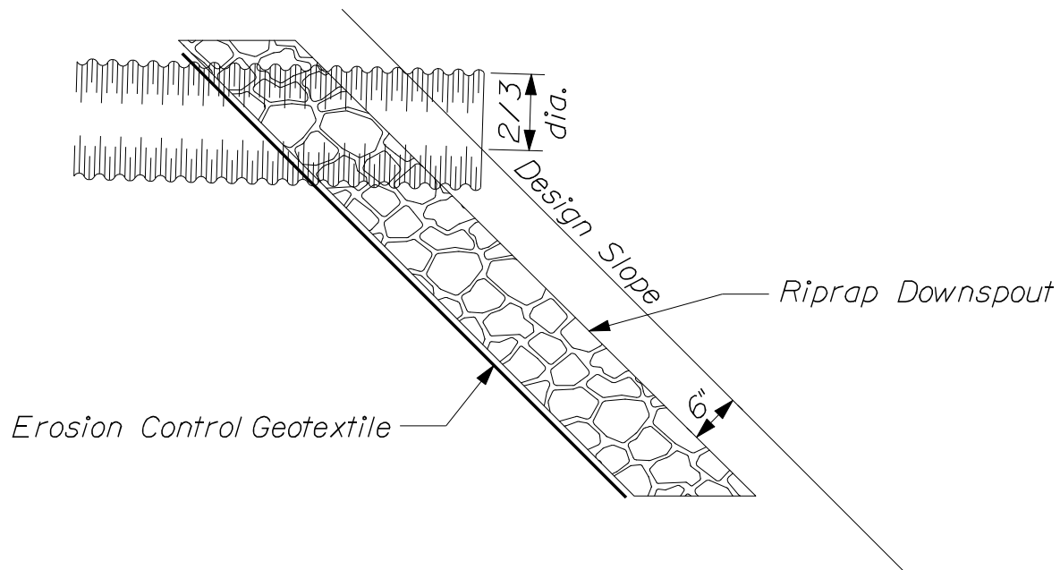
~ DETAIL I ~ TYPE "F" CATCH BASIN WITH OUTLET PIPE AND RIPRAP 604(II)
